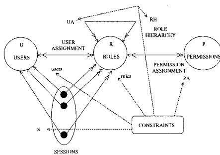
Figure 1 RBAC Model
