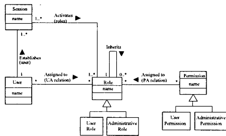
Fig.2: Conceptual Class Model for RBAC - entity classes
