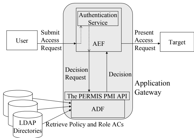
Figure 2. The Privilege Verification Subsystem
