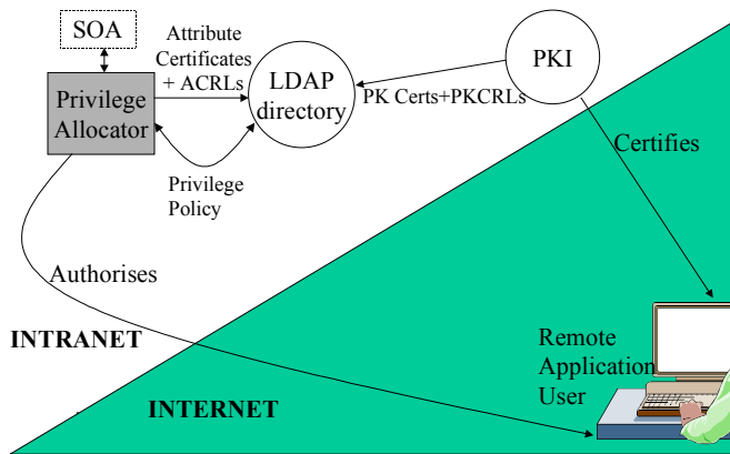
Figure 1. The Privilege Allocation Subsystem
