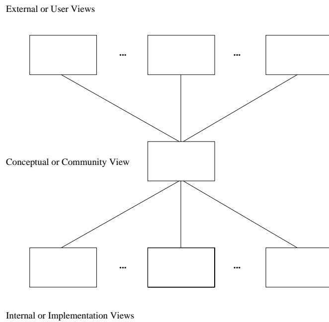
Figure 14: ANSI/SPARC Database Architecture
