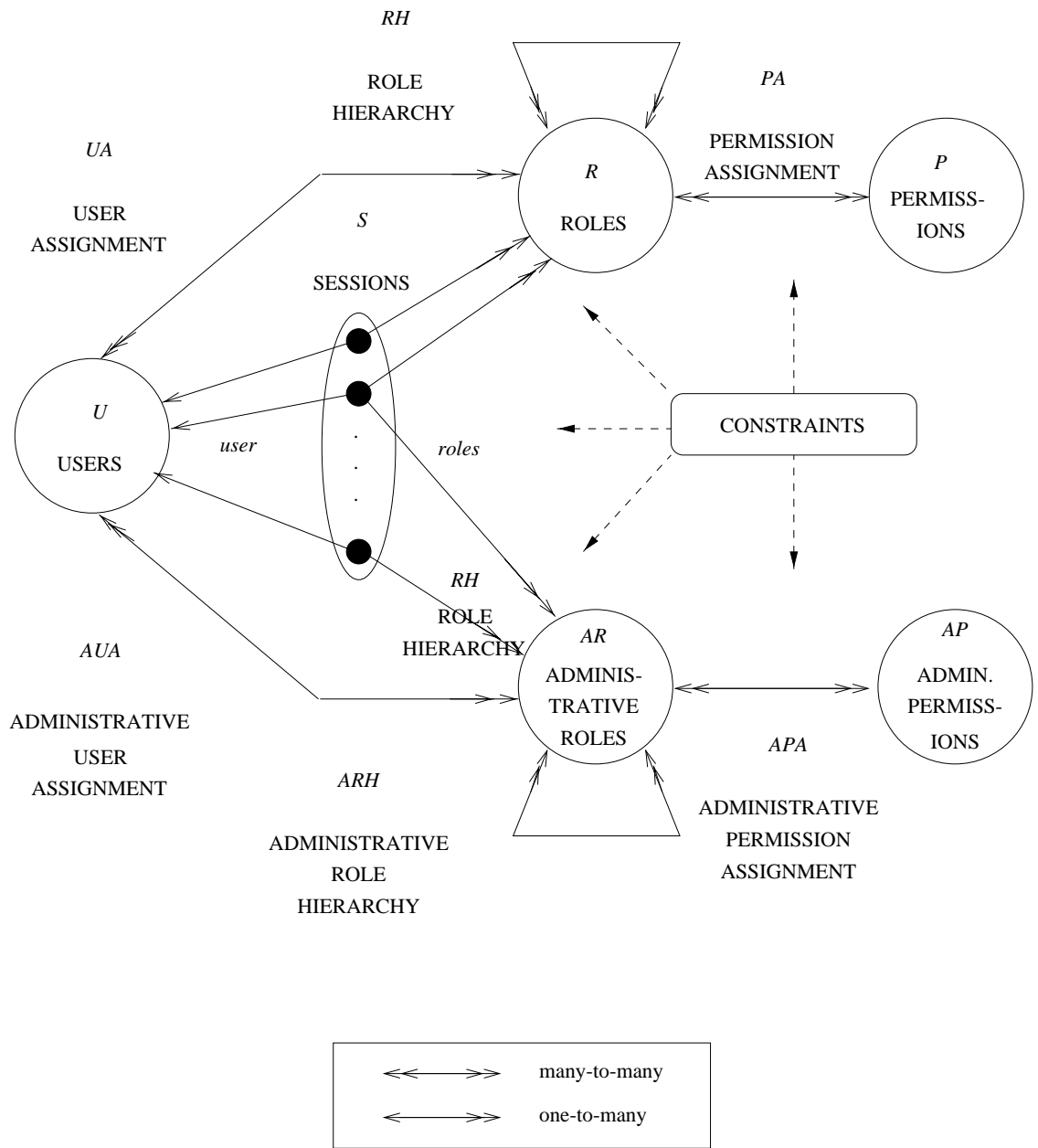
Figure 4: RBAC Administrative Model
