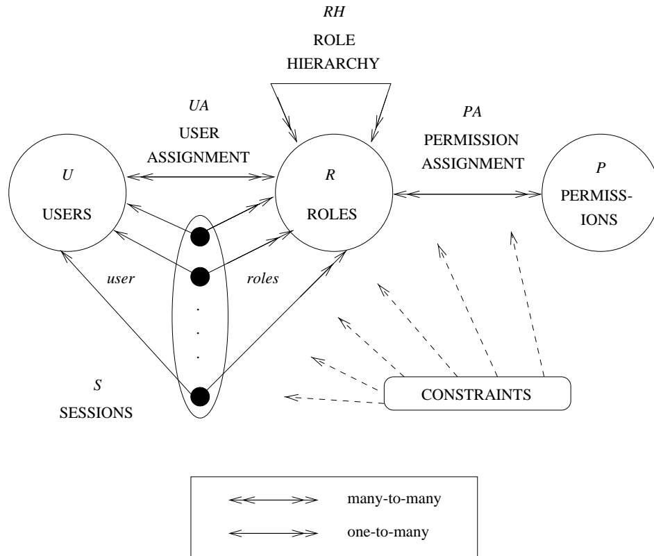
(b) The RBAC 3 model
