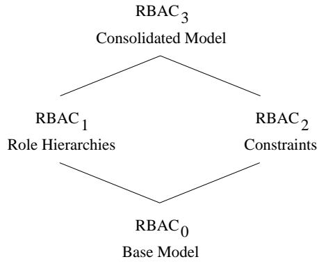
(a) Relationship among RBAC96 models
