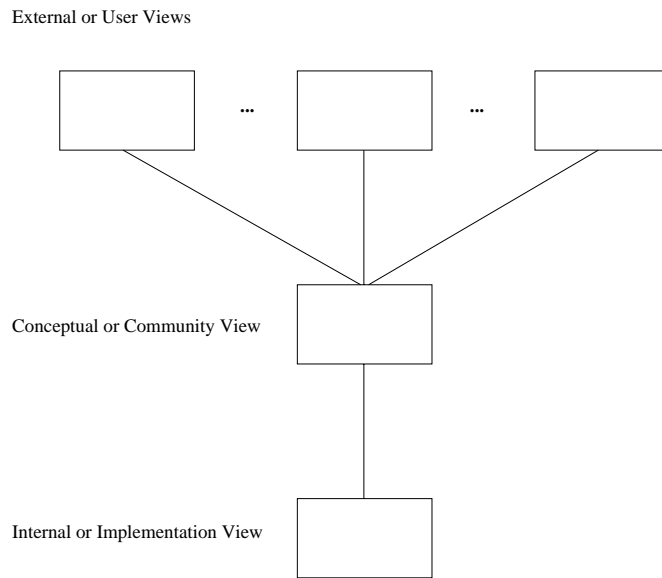
Figure 14: ANSI/SPARC Database Architecture
