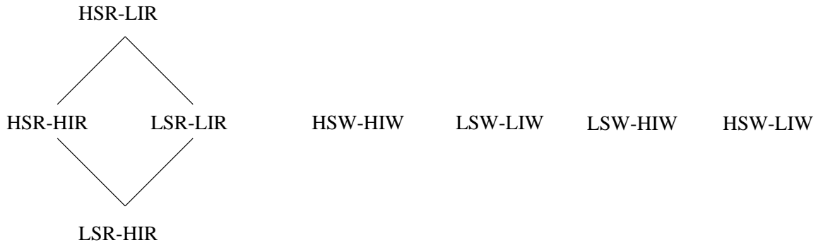
(c) Strict Confidentiality and Strict Integrity
